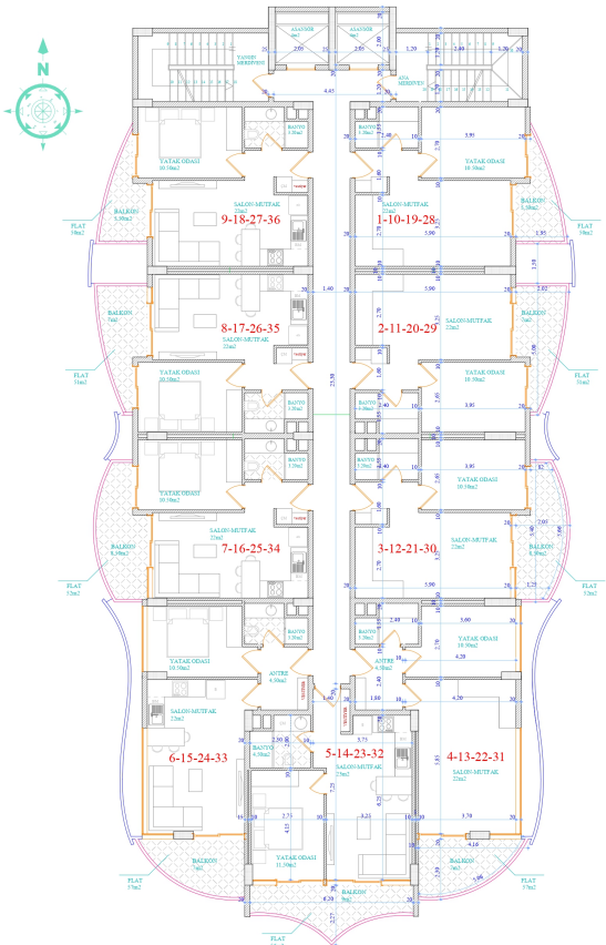
designed by: İLKER ÖMET KARADİMAN A BLOK NORMAL KAT PLANI
