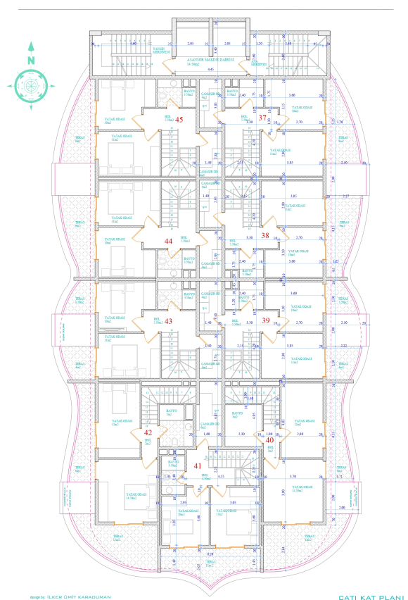
designed by: İLKER ÖMET KARADİMAN CATI KAT PLANI
