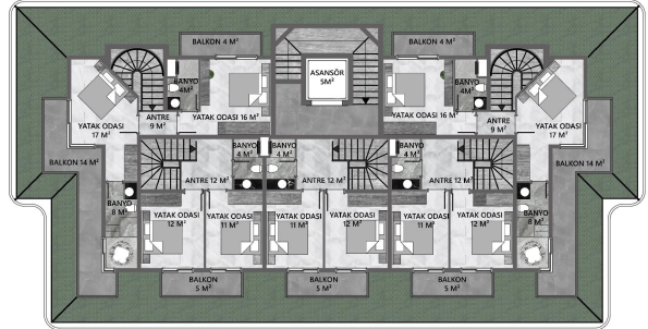
20 NOLU DUBLEX TOPLAM BRÜT: 132 M 2 NET: 124 M 2 19 NOLU DUBLEX TOPLAM BRÜT: 98 M 2 NET: 90 M 2 18 NOLU DUBLEX TOPLAM BRÜT: 98 M 2 NET: 90 M 2 17 NOLU DUBLEX TOPLAM BRÜT: 98 M 2 NET: 90 M 2 16 NOLU DUBLEX TOPLAM BRÜT: 132 M 2 NET: 124 M 2
