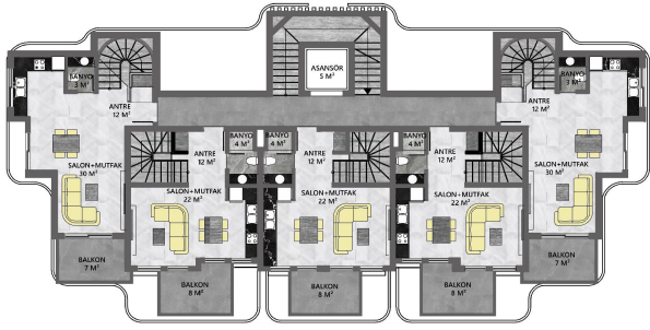
20 NOLU DUBLEX DAİRE BRÜT: 132 M 2 NET: 124 M 2 19 NOLU DUBLEX DAİRE BRÜT: 98 M 2 NET: 90 M 2 18 NOLU DUBLEX DAİRE BRÜT: 98 M 2 NET: 90 M 2 17 NOLU DUBLEX DAİRE BRÜT: 98 M 2 NET: 90 M 2 16 NOLU DUBLEX DAİRE BRÜT: 132 M 2 NET: 124 M 2
