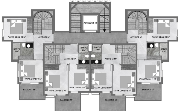
4 NOLU DUBLEX DAİRE BRÜT: 104 M 2 NET: 96 M 2 3 NOLU DUBLEX DAİRE BRÜT: 94 M 2 NET: 86 M 2 2 NOLU DUBLEX DAİRE BRÜT: 94 M 2 NET: 86 M 2 1 NOLU DUBLEX DAİRE BRÜT: 104 M 2 NET: 96 M 2
