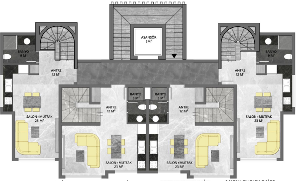
B BLOK BODRUM KAT PLANI
