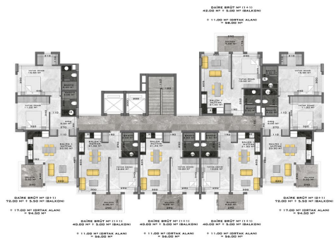
B - C BLOK NORMAL KAT PLANI
