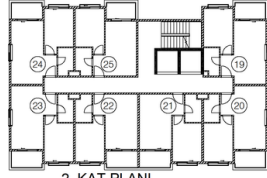
2. KAT PLANI
