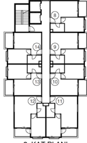
2. KAT PLANI
