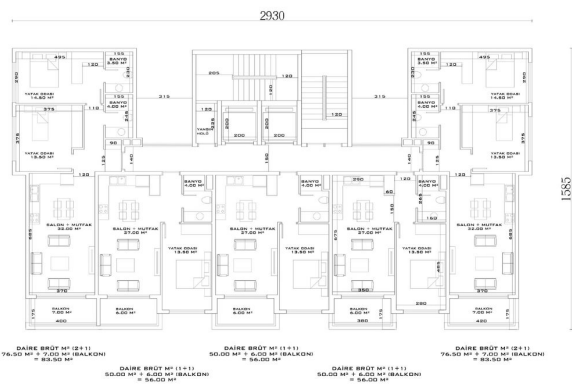
B - C BLOK NORMAL KAT PLANI
