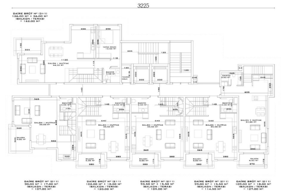
A - D BLOK DUBLEKS ALT KAT PLANI
