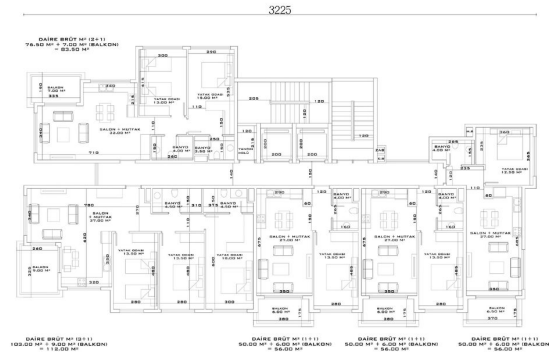
A - D BLOK NORMAL KAT PLANI
