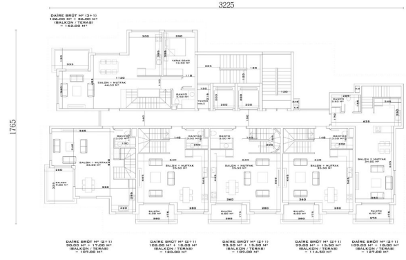
A - D BLOK DUBLEKS ALT KAT PLANI
