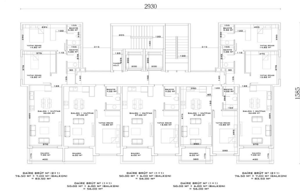
B - C BLOK NORMAL KAT PLANI
