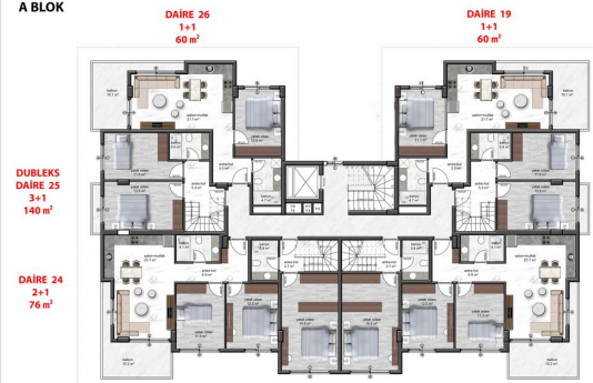
3.KAT PLANI
