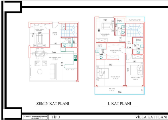
VILLA KAT PLANI
