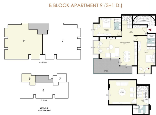
2. Floor and roof floor plan
