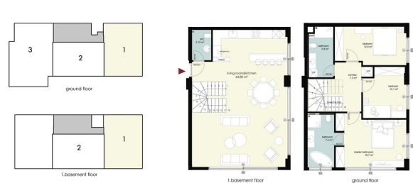
1. Basement and ground floor plan
