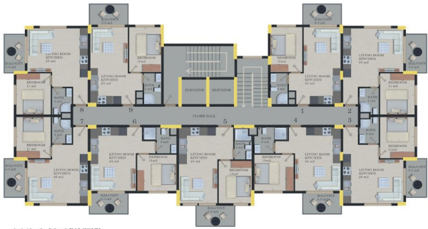
1-2-3-4-5-6 FLOOR PLAN
