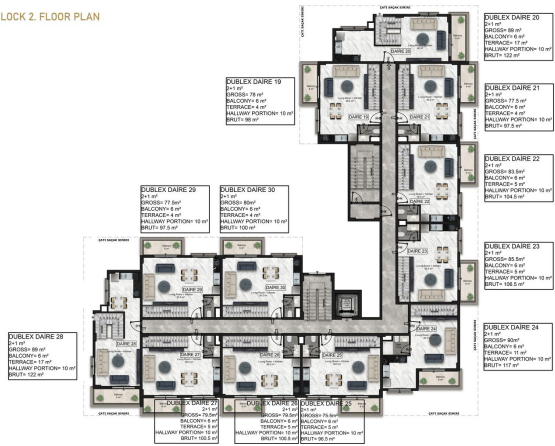
6 BLOCK 2 FLOOR PLAN
