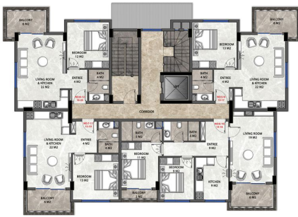
1-2-3-4 FLOOR PLAN
