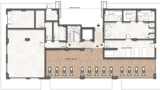
A BLOK 1.BODRUM KAT PLANI
