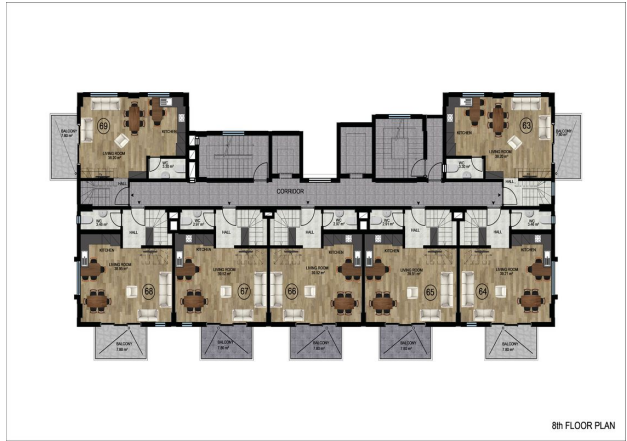
8th FLOOR PLAN
