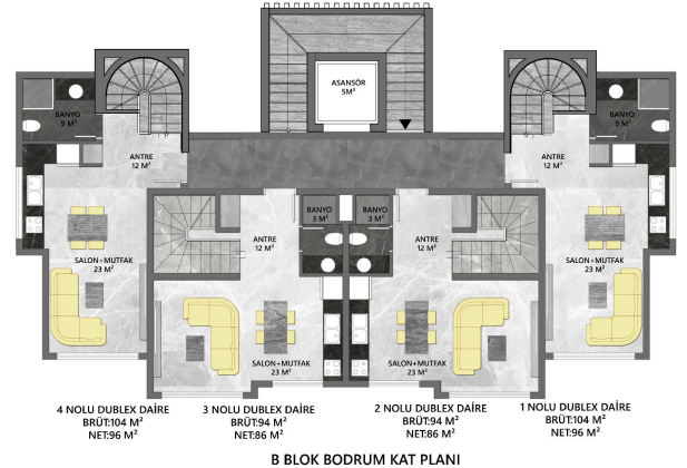
B BLOK BODRUM KAT PLANI
