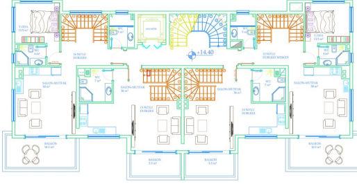
DUBLEX ALT KAT PLANI
