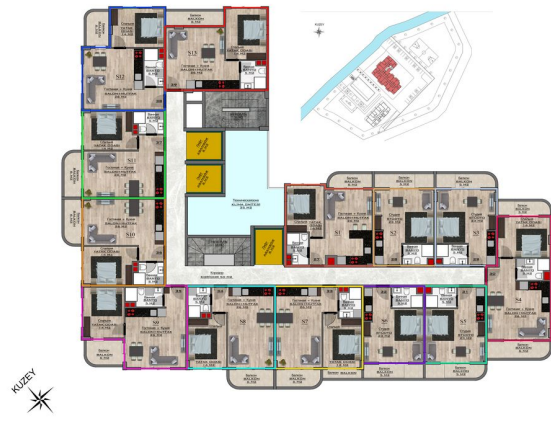
2. KAT PLANI
