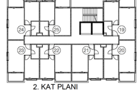
2. KAT PLANI
