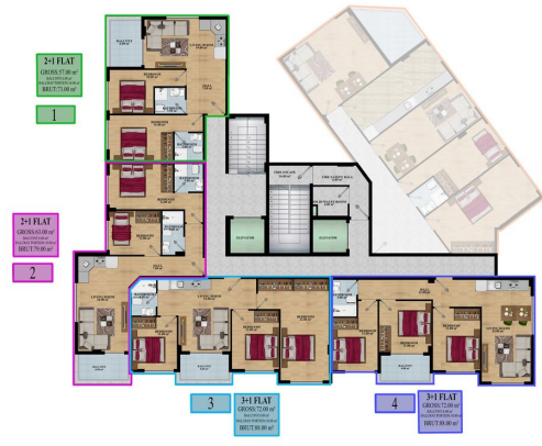
-1 BASEMENT FLOOR PLAN
