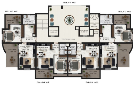
C BLOK GROUND FLOOR PLAN (NORMAL KAT) SCALE 1/50
