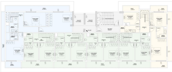
A BLOK ÇATI KATI PLANI
