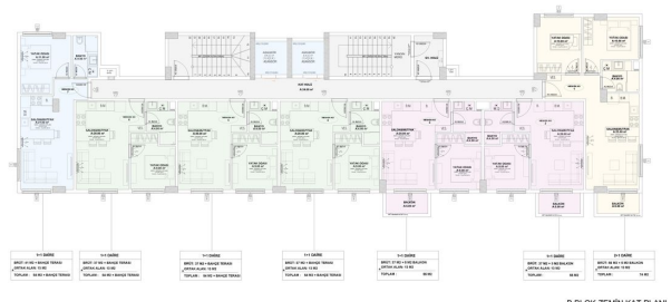
B BLOK ZEMIN KAT PLAN
