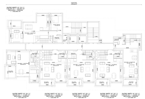
A - D BLOK DUBLEKS ALT KAT PLANI
