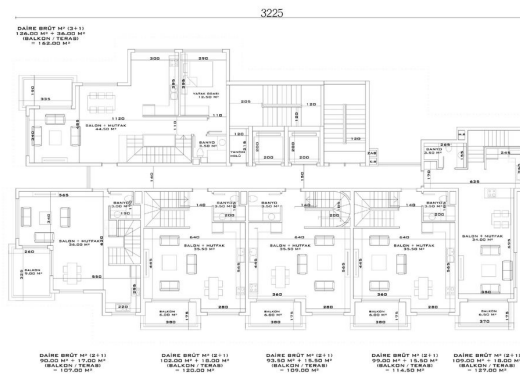
A - D BLOK DUBLEKS ALT KAT PLANI
