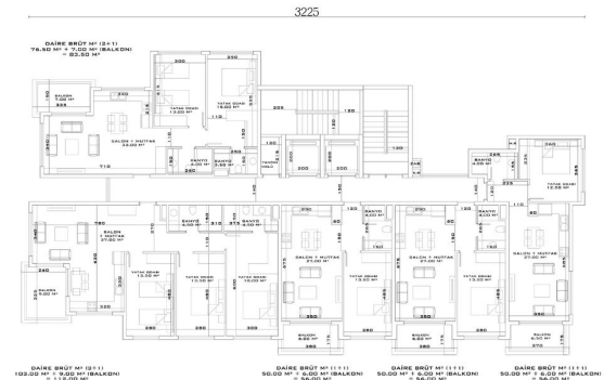
A - D BLOK NORMAL KAT PLANI
