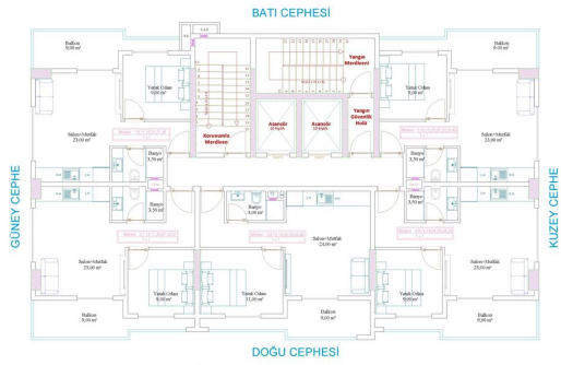
B BLOK ZEMİN, 1, 2, 3, 4, 5, 6, 7. KAT PLANI
