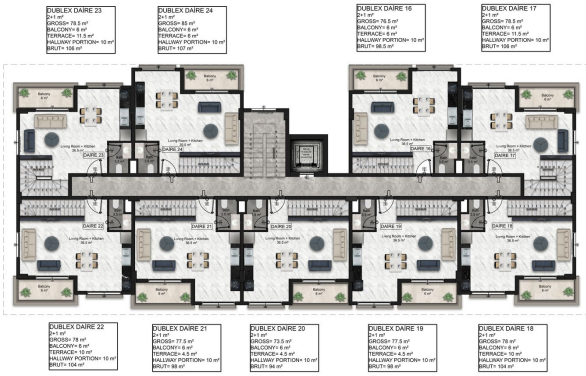
A-B-C-D-E-F BLOCK 2. FLOOR PLAN
