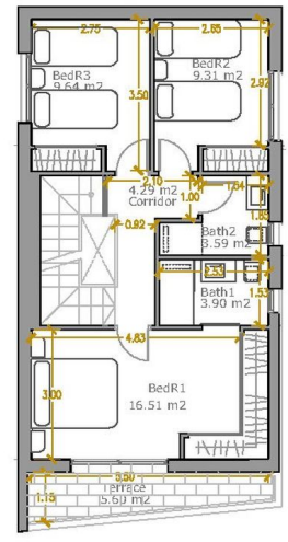
THIRD FLOOR
