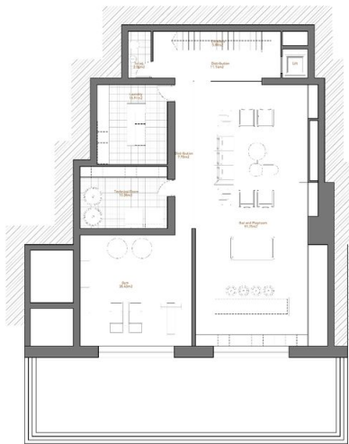
LEVEL +148.60 (Basement)
