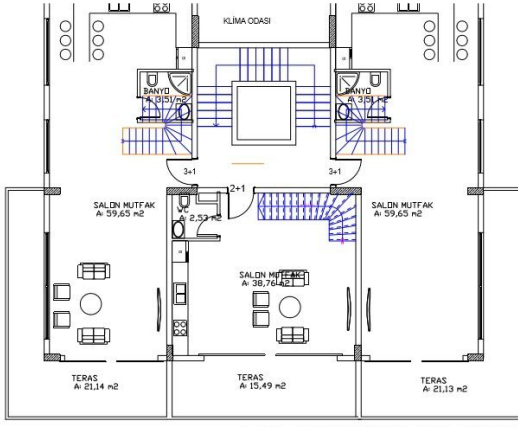
TERS DUBLEKS ALT KAT PLANI
