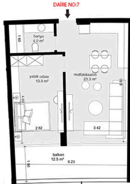
E BLOCK - GROUND FLOOR PLAN
