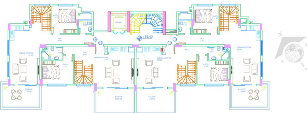
DUBLEX ALT KAT PLANI
