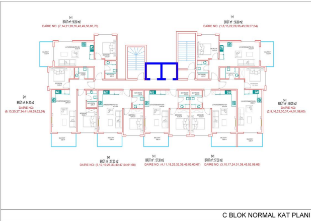
C BLOK NORMAL KAT PLANI
