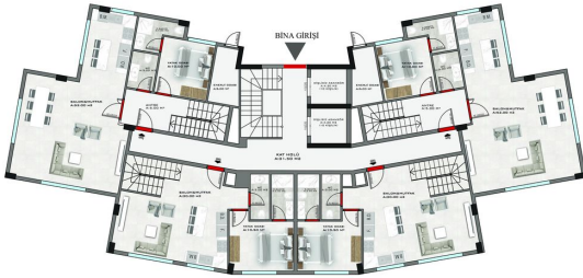
1159/1 KESTEL / B BLOK -1 BODRUM KAT PLANI
