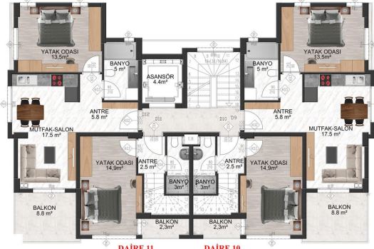
DAİRE 11 3+1 DUBLEX 29 m 2 +96 m 2 = 125 m 2
