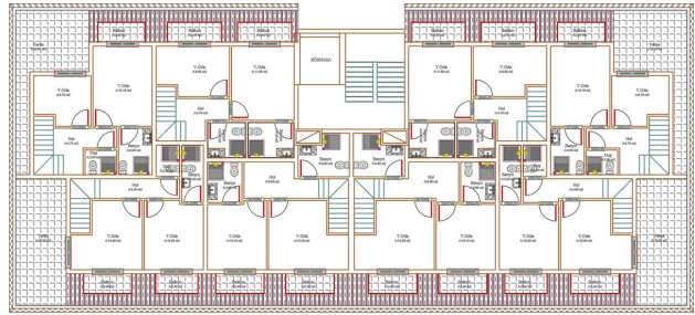
ÇATI KAT PLANI
