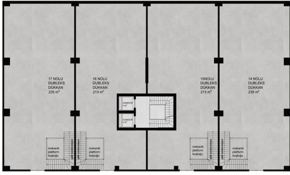
B BLOK /-1. BODRUM KAT PLANI
