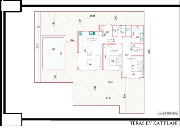
TERAS EV KAT PLANI
