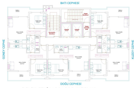
B BLOK ZEMİN, 1, 2, 3, 4, 5, 6, 7. KAT PLANI
