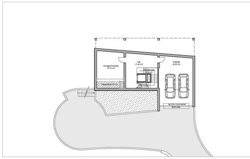
BASEMENT FLOOR
